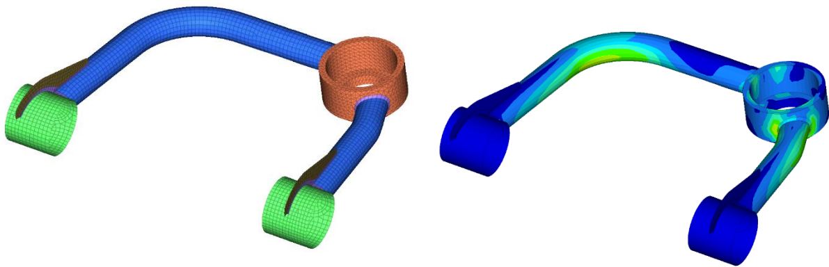
Figure 2: Upper Control Arm Mesh and Stress Contour
