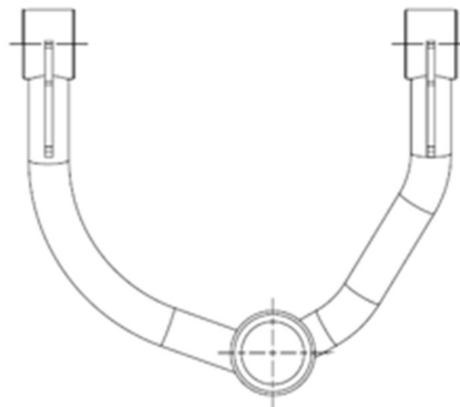
Figure 1: Upper Control Arm Design
