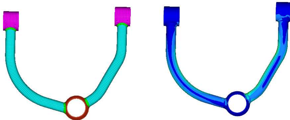
Figure 2: Upper Control Arm Mesh and Stress Contour
